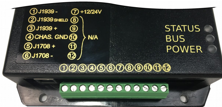
Figure 1: TMT7839 Terminal Strip
